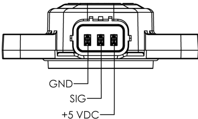
1878 Pinout Diagram
